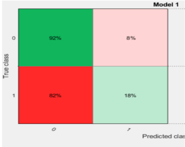
Fig 2: Decision Tree True positive rate and false negative rate
