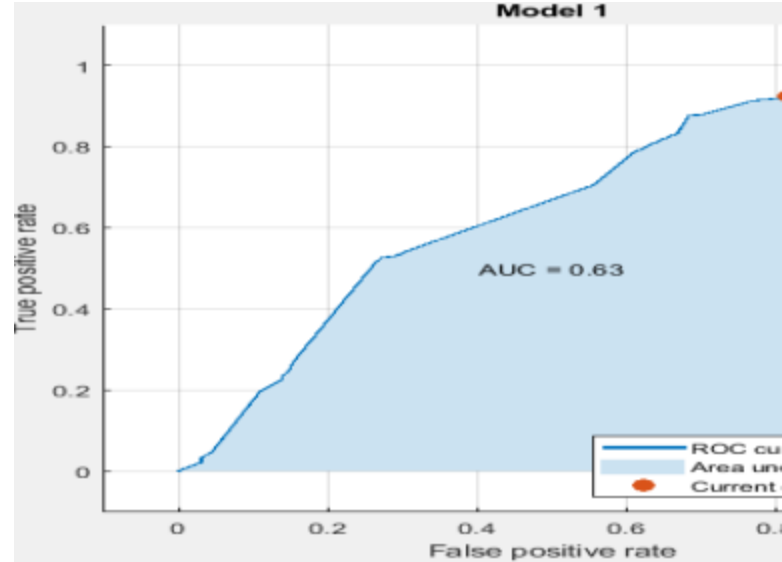
Fig 4: Decision Tree ROC curve
